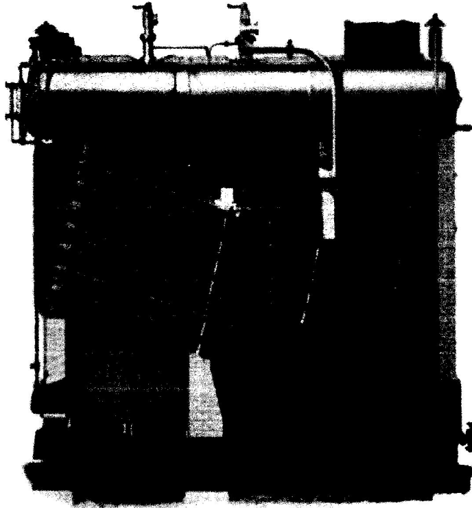
Figure 2.6 Babcock and Wilcox water tube boiler with longitudinal steam drum
