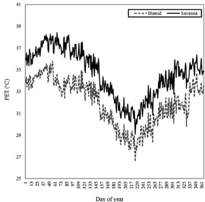
Fig. 3 Mean daily physiologically equivalent temperature pattern in humid forest (Okitipupa) and derived savannah (Akoko Southwest) ecoclimatic zones of Ondo State, Nigeria (1998–2008)
