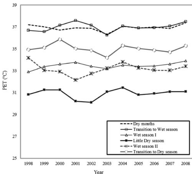
Fig. 5 Annual course of physiologically equivalent temperature in different seasons in derived savannah (Akoko Southwest) ecoclimatic zone of Ondo State, Nigeria (1998–2008)
