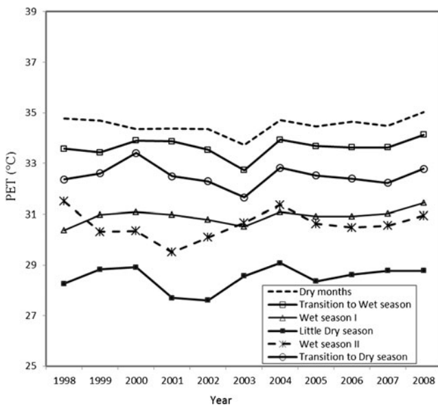
Fig. 4 Annual course of physiologically equivalent temperature in different seasons in humid forest (Okitipupa) ecoclimatic zone of Ondo State, Nigeria (1998–2008)
