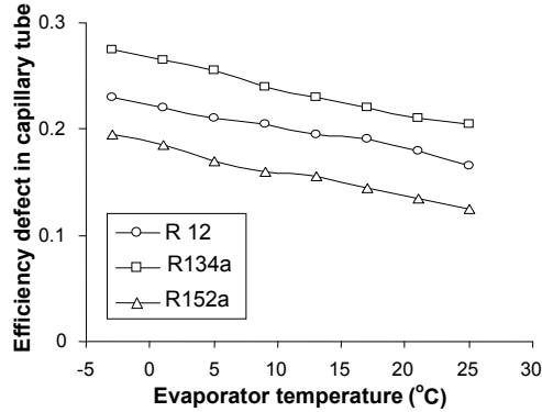
Fig. 7. Variation of Efficiency Defect in Capillary Tube with Evaporator Temperature.
