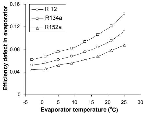
Fig. 8. Variation of Efficiency Defect in Evaporator with Evaporator Temperature.
