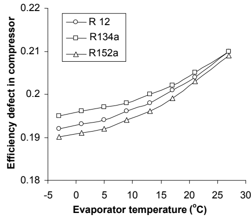
Fig. 5. Variation of Efficiency Defect in Compressor with Evaporator Temperature.
