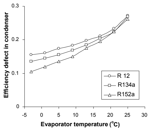
Fig. 6. Variation of Efficiency Defect in Condenser with Evaporator Temperature.
