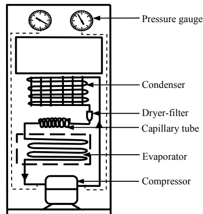
Fig. 2. Schematic Diagram of Experimental Refrigerator.
