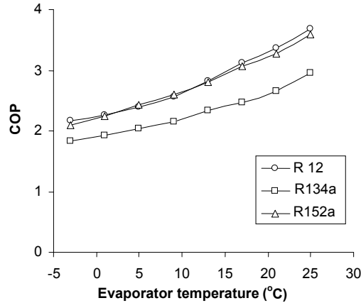
Fig. 3. Variation of Coefficient of Performance (COP) with Varying Evaporator Temperature.
