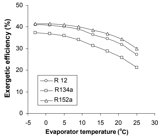
Fig. 4. Variation of Exergetic Efficiency with Evaporator Temperature.
